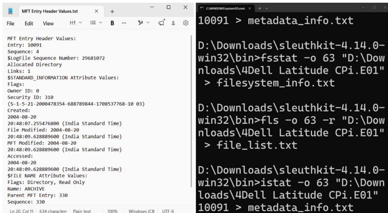
Figure 5: Viewing detailed file metadata (istat output) for inode 10091
